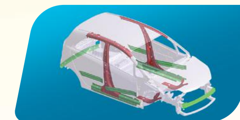
Reinforced Body Structure with Hot Press Formed Steel
